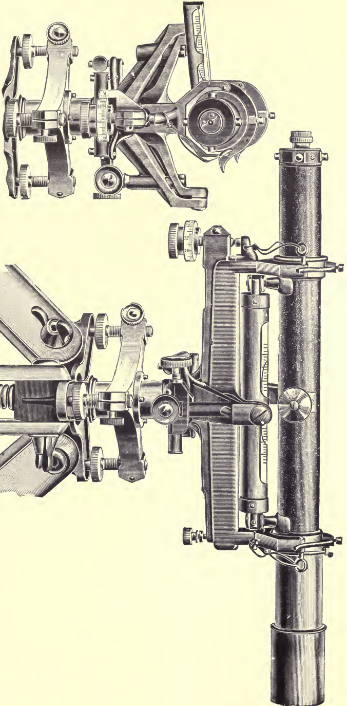
End view, showing Pivots and Fine Mirror with Universal Joint.
